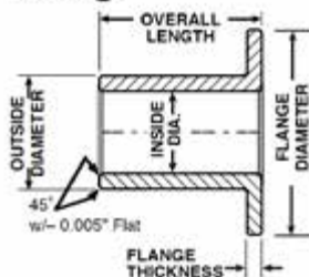
Flanged Bearings
