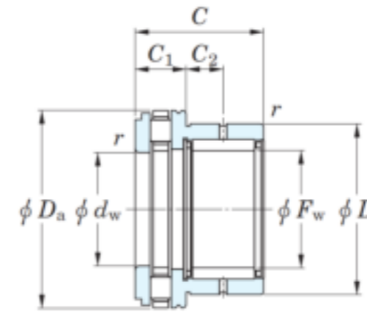
NAXR
