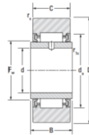
NA22.2RS.DZ
