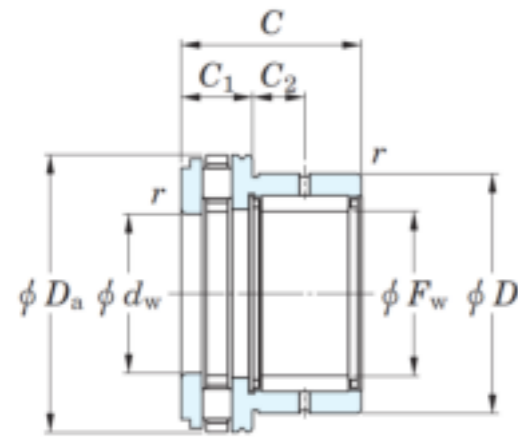
NAXR
